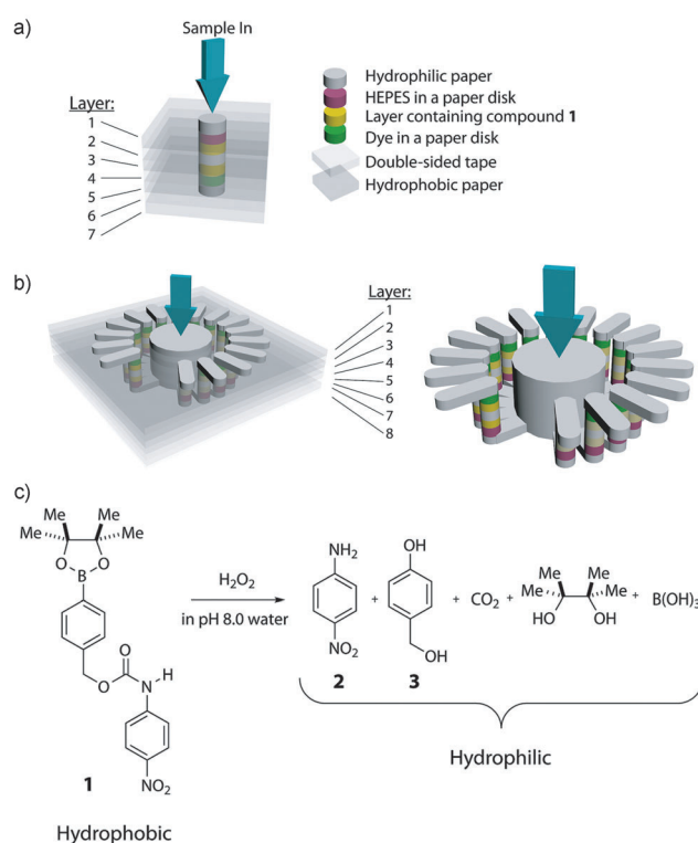
Figure 1. Two 3D paper-based microfluidic devices that are configured to quantify the level of hydrogen peroxide in a sample by simply measuring time. a) Digital assays that use a single conduit device to report the concentration of hydrogen peroxide by measuring the time required for the sample to flow through the device in the z direction. b) Analog assays that use a radial paper-based microfluidic device for quantifying the level of hydrogen peroxide by using a fixed assay time and by counting the number of bars that become colored as a function of the concentration of hydrogen peroxide in the sample. c) Both devices contain compound 1 , which modulates the wetting properties of defined hydrophilic regions in the devices in a dose-dependent manner when exposed to hydrogen peroxide. Oxidative cleavage of 1 (which is hydrophobic) by hydrogen peroxide yields hydrophilic products and changes the wetting properties of layers 3 and 5 (a, b).
